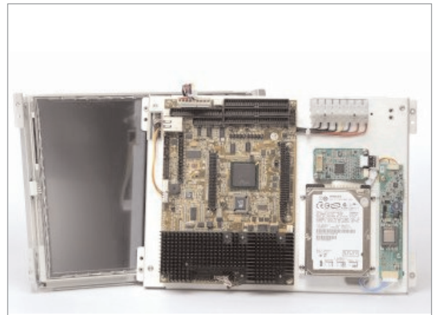
WinSystems' Flat Panel Open Frame Mount
