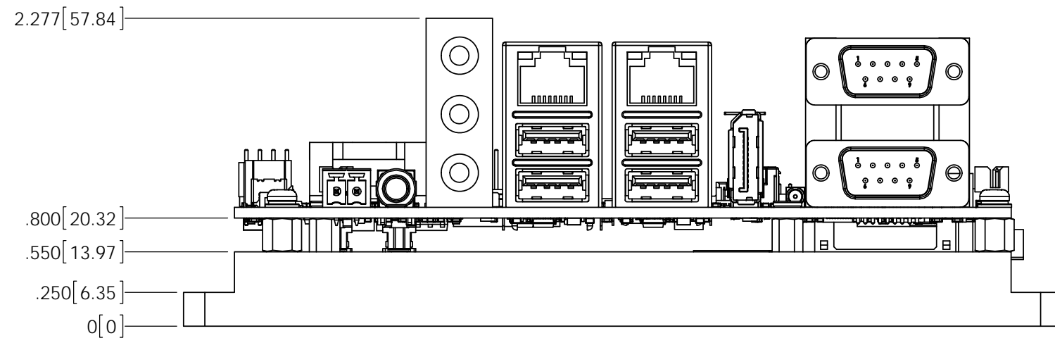
CC405 - COMe MECHANICAL
